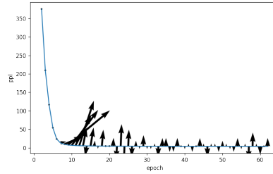
Fig. 3. Actual ppl change during training. The very first epoch is deleted for better visualization without changing the shape of the curve. The curvature is visualized as black arrows.
